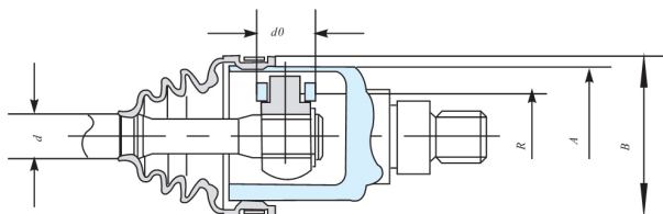
Boundary dimensions of TJ type universal joints
