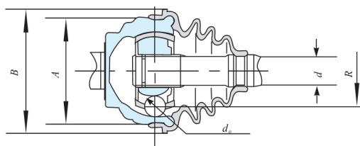
Boundary dimensions of BJ type universal joints
