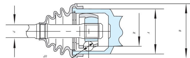
Boundary dimensions of DOJ type universal joints
