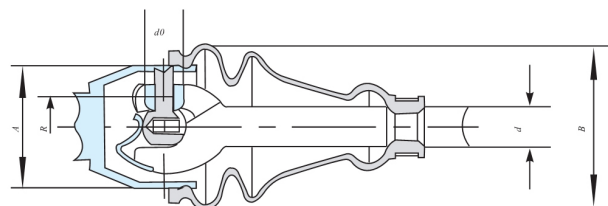
Boundary dimensions of GE type universal joints
